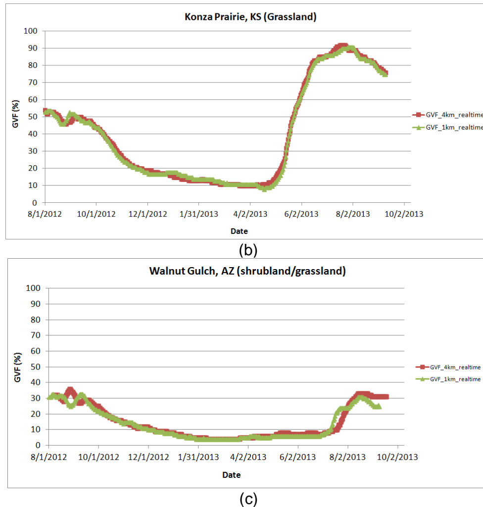
Figure 13. Time series of 4-km and 1-km daily rolling weekly GVF at (a) Bondville (lat 40.00°, lon -88.29°), (b) Konza Prairie (lat 39.08°, lon -96.56°) and (c) Walnut Gulch (lat 31.737°, lon -109.942°).
