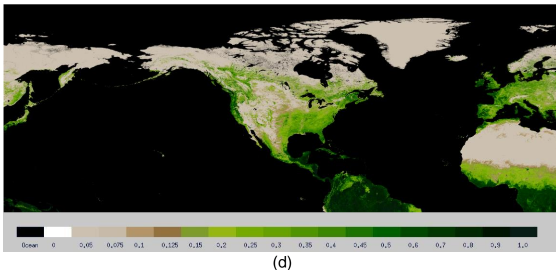
Figure 12. Daily rolling weekly Green Vegetation Fraction maps produced by the GVFP system: (a) Global 4-km GVF for the week of 8/4/2013-8/10/2013 (b) Regional 1-km GVF for the week of 8/4/2013-8/10/2013, (c) Global 4-km GVF for the week of 2/14/2013-2/20/2013, and (d) Regional 1-km GVF for the week of 2/14/2013-2/20/2013.
