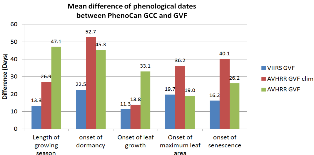
Figure 22. Mean difference of phenological dates between PhenoCan GCC and GVF.
